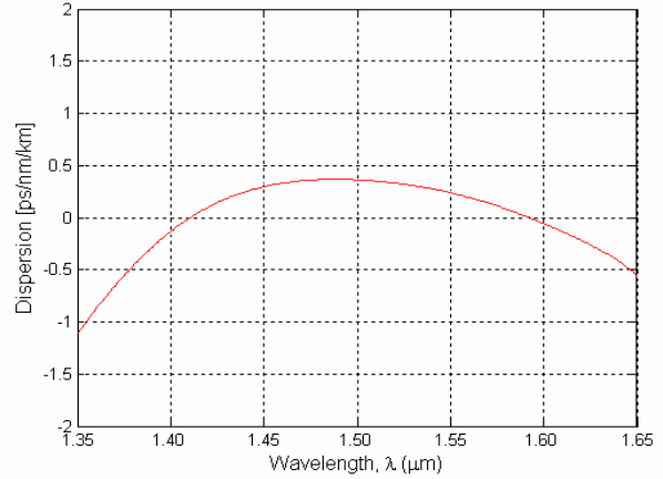
Fig.5 Dispersion characteristics of the DF-PCF for \Lambda_1 = 2.30 \mu\text{m} , d_1/\Lambda_1 = 0.28 , and d_2/\Lambda_1 = 0.58 .
