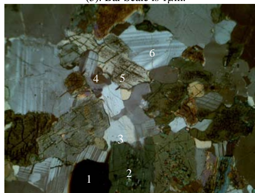
Fig. 7: Photomicrograph of Charnockite (Ak007b a) showing hornblende (1), biotite (2), quartz (3), zircon (4), hypersthene (5) and plagioclase (6). Bar Scale is 2µm.
