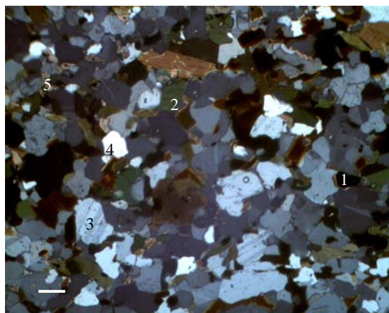
Fig. 8: Photomicrograph of Hybrid rock (H1 c) showing hornblende (1), biotite (2), plagioclase (3), quartz (4) and hypersthene (5). Bar Scale is 1 \mu m.
