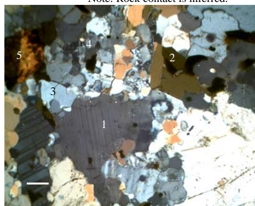
Fig. 6: Photomicrograph of Porphyritic granite (Pgr b) showing plagioclase (1), biotite (2), quartz (3), microcline (4) and orthoclase (5). Bar Scale is 1µm.
