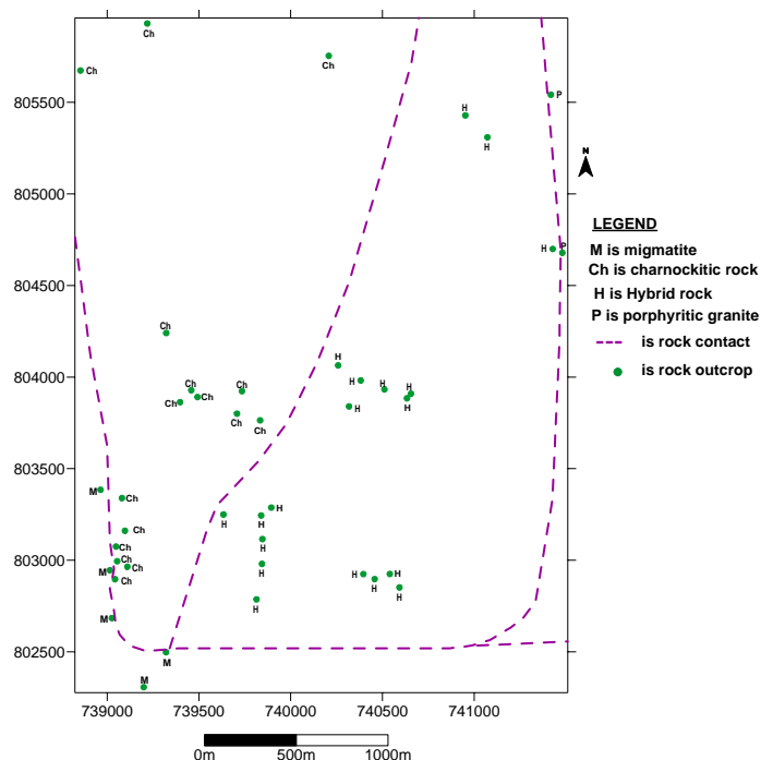
Fig. 5: Plots of outcrops locations in the study area (coordinates converted to UTM with Transfo and plotted in Surfer 8). Note: Rock contact is inferred.
