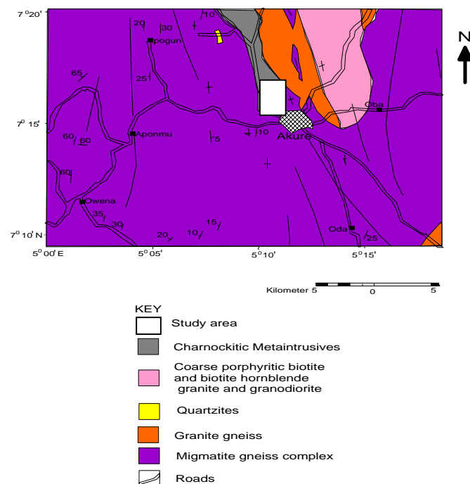
Fig.1: Geological Map of Akure showing study Area (Adapted from Ademeso, 2009)
