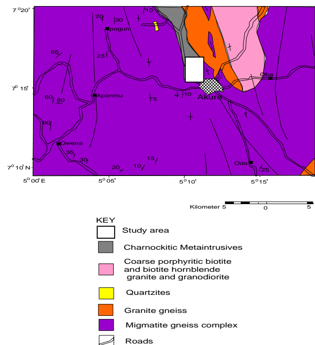
Fig.1: Geological Map of Akure showing study Area (Adapted from Ademeso, 2009)
