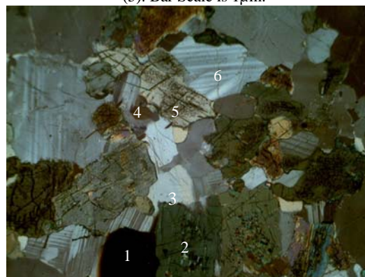
Fig. 7: Photomicrograph of Charnockite (Ak007b a) showing hornblende (1), biotite (2), quartz (3), zircon (4), hypersthene (5) and plagioclase (6). Bar Scale is 2µm.
