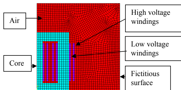
Fig. 2 Schematic of transformer with elements
