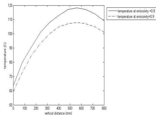
Fig. 10 Distribution of temperature at different emissivities
