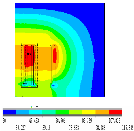
Fig. 5b Calculated temperature distribution at ambient 30°C
