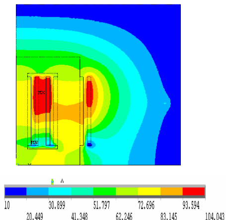
Fig. 5a Calculated temperature distribution at ambient 10°C
