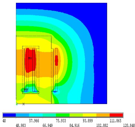
Fig. 3 Calculated temperature distribution at full load 800 kVA
