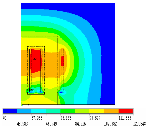
Fig. 9a Calculated temperature at emissivity 0.8
