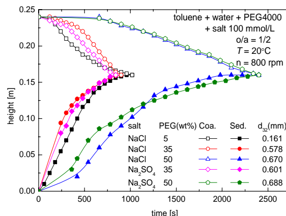
Fig. 6 Comparison of coalescence and sedimentation curve of o/a = 1/2 at different concentrations of PEG4000 and 100 mmol/L \text{NaCl} and \text{Na}_2\text{SO}_4
