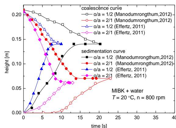
Fig. 4 Coalescence and sedimentation curve of MIBK-water system o/a = 1/2 and 2/1 [6]-[7]
