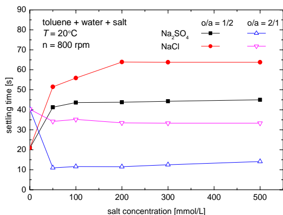
Fig. 5 Influence of salt on the settling time
