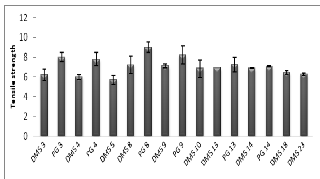
Fig. 1 Tensile strength in DMS and PG containing patches
