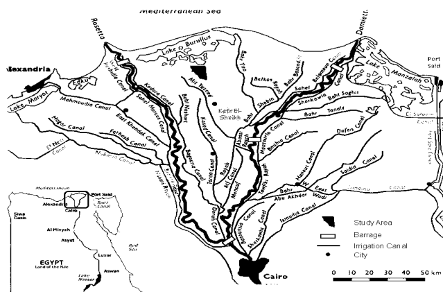
Fig. 1 layout of irrigation networks in The Nile Delta's area
