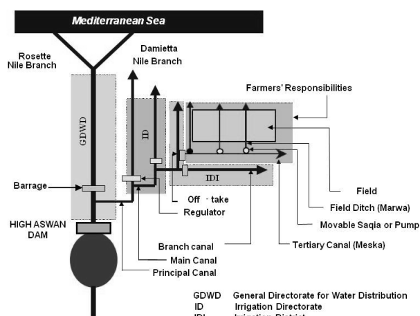
Fig. 2 schematic layout of irrigation systems in Nile Delta Egypt
