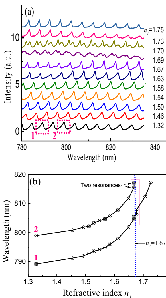
Fig. 5 (a) Evolution of the fluorescence spectrum, starting from methanol ( n_1=1.32 ), and subsequently pumping oils into the channel with nominal refractive indices ranging from 1.46 to 1.75. The spectral shift of two peaks centered at \lambda = 789.95 nm and 798.97 nm, respectively, for n_1 = 1.32 re traced out in (b). The dashed line marks the refractive index value of the QD film. The square encompasses the range of refractive indices for which two families of modes were observed. The lines connecting the points are a guide to the eye
