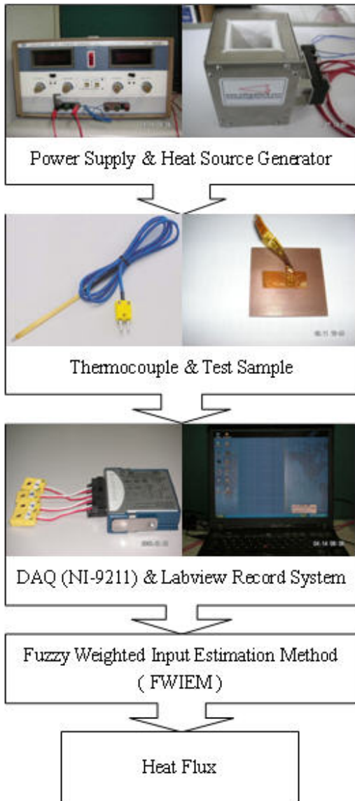
Fig. 1. The structure chart of the experiment.
