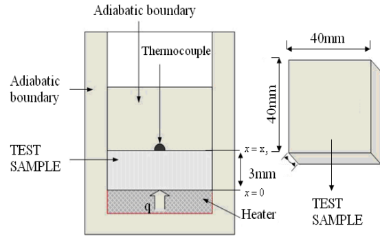
Fig. 2. The heat-conducting model.
