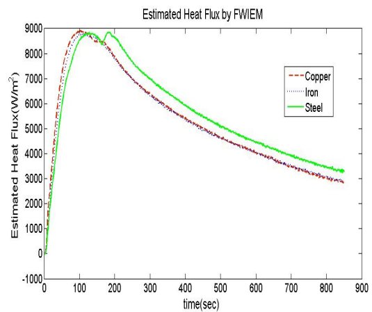
Fig. 4. The curves of estimated heat flux.
