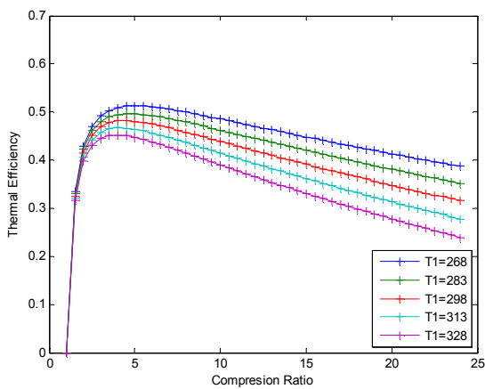
Fig. 6 Effect of compression ratio and ambient temperature on thermal efficiency (specified TIT).
