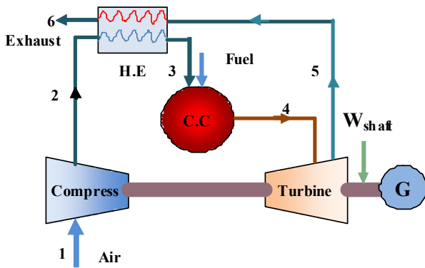
Fig. 1 The regenerative gas turbine cycle.
