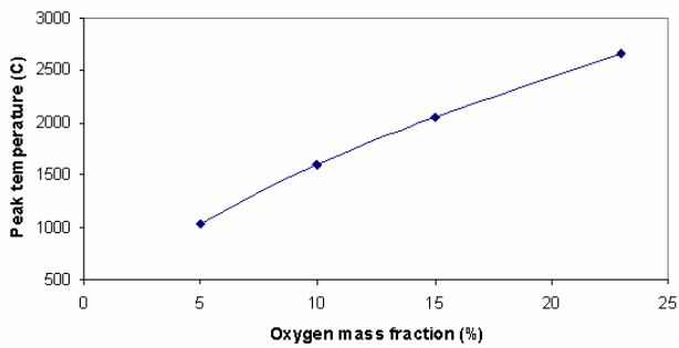
Fig. 5 The variations of peak temperature at various oxygen concentrations in HiTAC's temperature
