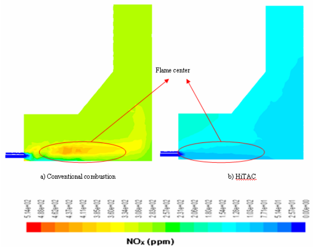
Fig. 7 The NOx concentration contour plots in the conventional combustion and HiTAC
