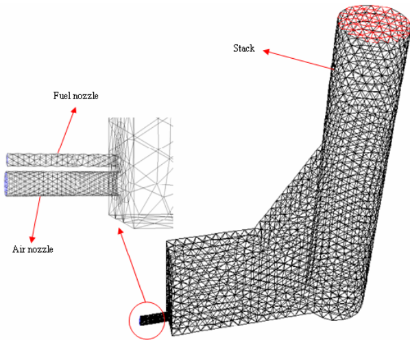
Fig. 1 The modeled combustion chamber with a burner
