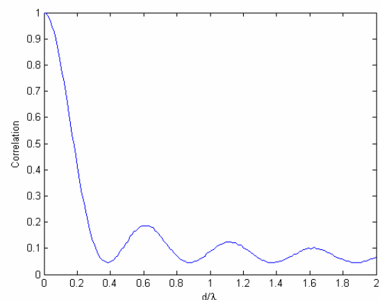
Fig. 2 Correlation vs. distance between antenna at receiver (SNR=20 dB)
