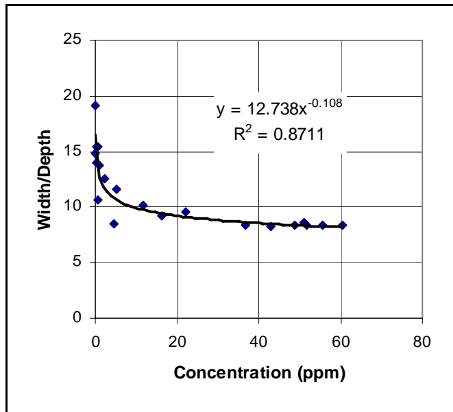
Fig. 2 The relation between shape factor ( w/d ) and sediment transport for Yalobosha River by using equation 26 (Shen and Hung, 1971)
