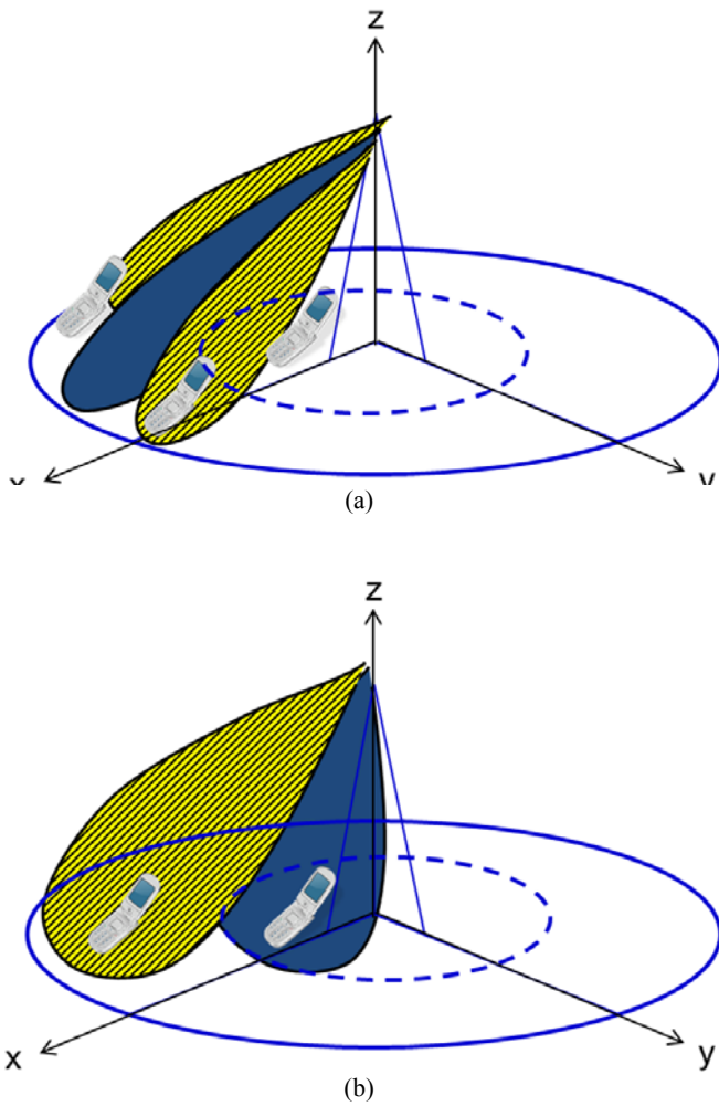
Fig. 3 (a) Horizontal and (b) vertical beamforming
