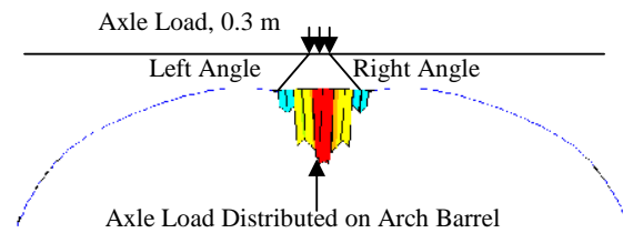
Fig. 13 Axle Load Distribution, at Crown
