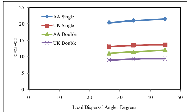
Fig. 2 Load vs Dispersal Angle, Griffith Bridge
