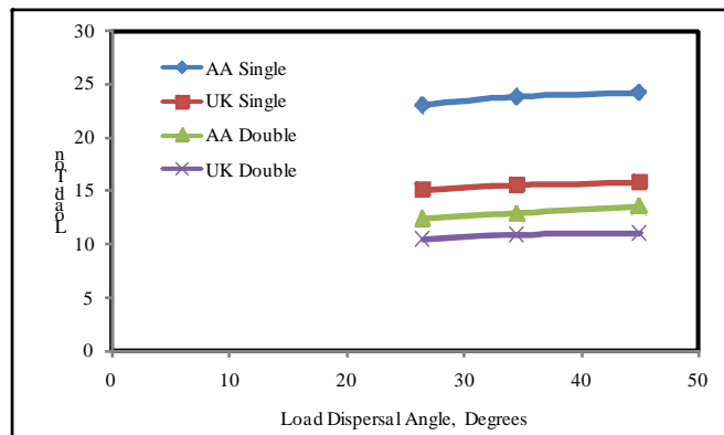
Fig. 3 Load vs Dispersal Angle, Killeen Bridge
