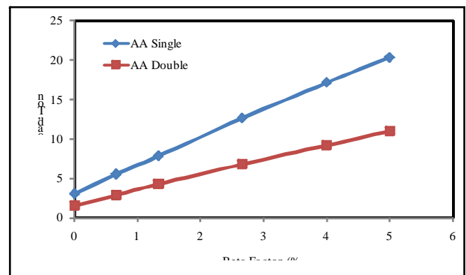
Fig. 6 The Effect of Arch \beta factor, Killeen Bridge
