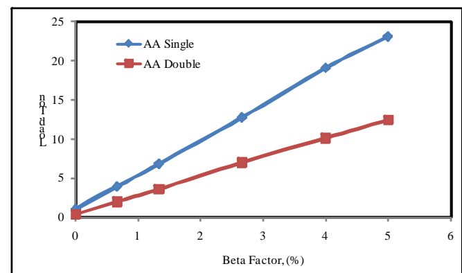
Fig. 7 The Effect of Arch \beta factor, Griffith Bridge
