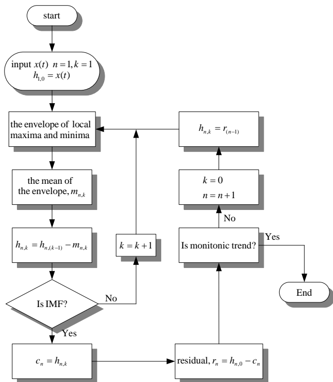
Fig. 1 The flowchart of EMD.
