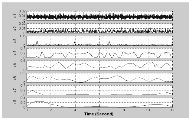
Fig. 3(a) Time-amplitude distribution of Sample 2
