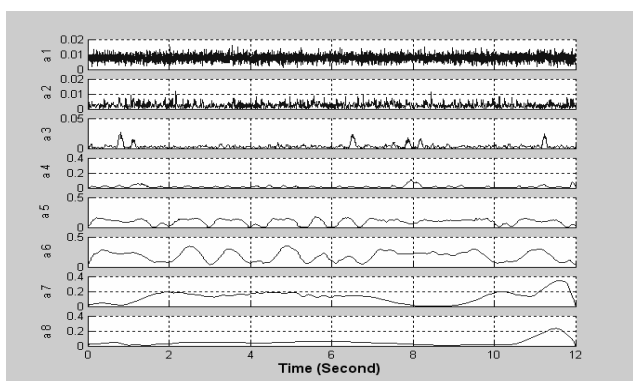
Fig. 3(b) Time-amplitude distribution of Sample 4
