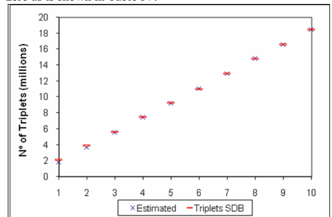
Fig. 7. Formula validation.
