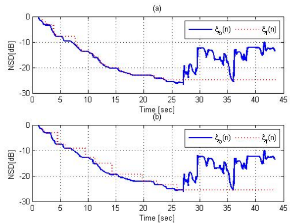
Fig. 6 NSD of background filter (solid line) and foreground filter (dotted line) for the ITP and proposed solution in a doubletalk situation. Doubletalk occurs after 26 s. (a) NSD for the ITP, \alpha_{b, f} = 0\text{dB} . (b) NSD for the proposed solution, \alpha_0 = 0\text{dB}
