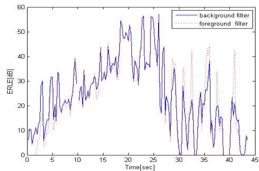
Fig. 7 ERLR of background filter (solid line) and foreground filter (dotted line) for the proposed solution in a doubletalk situation. Doubletalk occurs after 26 s
