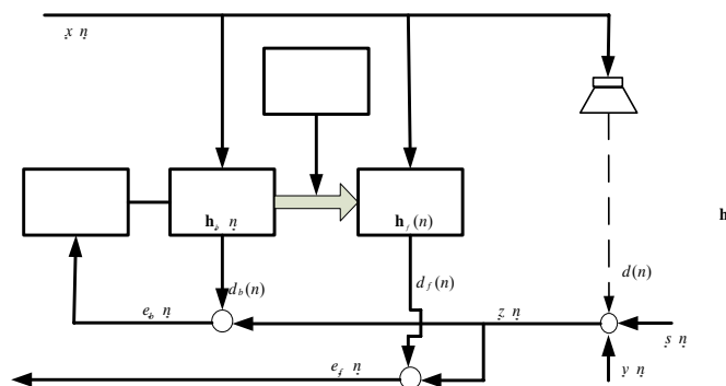
Fig.1 Two-path structure
