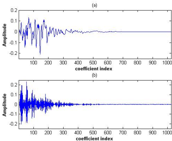
Fig. 4 Echo paths (a) h_1 . (b) h_2
