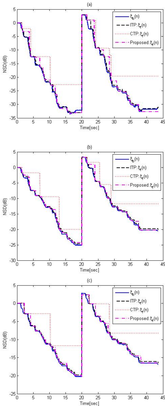
Fig. 8 NSD comparison of the CTP, ITP and proposed solutions for different step-size in the echo path change situation. Echo path change occurs from \mathbf{h}_1 to \mathbf{h}_2 at 20 s
