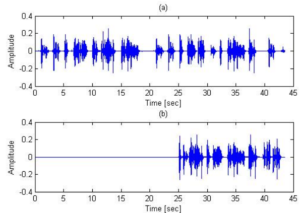
Fig. 3. Speech signals. (a) Far-end signal. (b) Near-end signal. Double talk occurs at about 26s.
