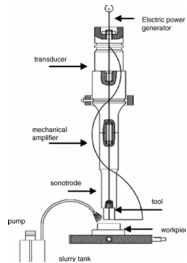
Fig. 1 USM Set Up
