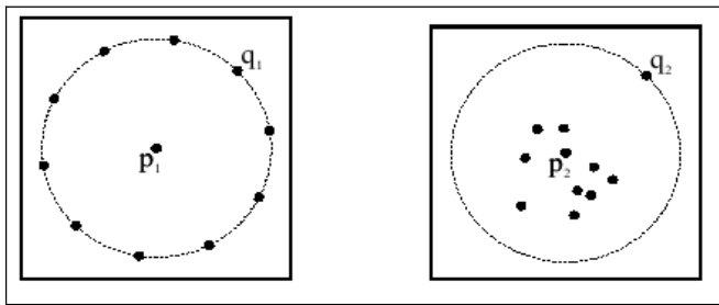
Fig. 2: The difference between Distance-based Outliers definitions. Both of p_1 and p_2 have 10 neighbors, in some approaches p_1 and p_2 have the same outlier ranking and in other approaches p_1 has larger outlier ranking than p_2
