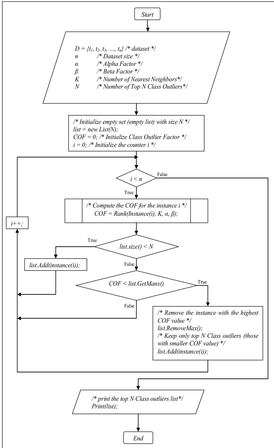
Fig. 12: The CODB algorithm flowchart
