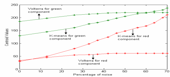
Fig. 5 Noise resistance curve
