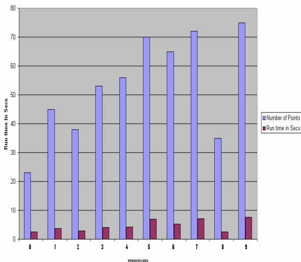
Fig. 4 Performance of DBSCAN Algorithm
