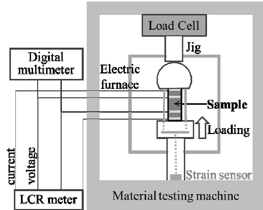
Fig. 1 Experimental setup for compressive test at elevated temperature
