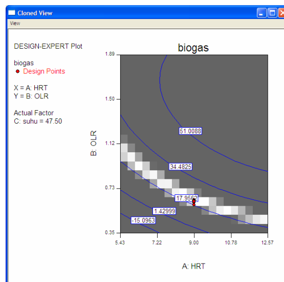
Fig. 1 Contour graph for biogas yield
