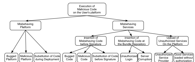
Fig. 5 The Attack Tree for malicious Code Execution
