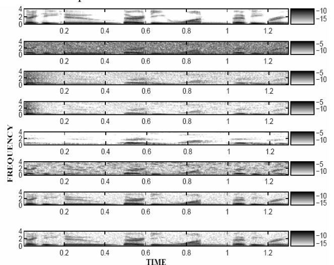
Fig. 7 Spectrogram of: (a) clean speech (b) speech corrupted by CIN at 0dB SNR (c) Me-1 enhanced speech (d) Me-2 enhanced speech (e) Me-3 enhanced speech (f) Me-4 enhanced speech (g) Proposed 1 enhanced speech (h) Proposed 2 enhanced speech
