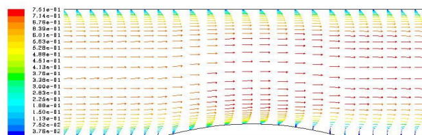
Fig. 4 Distribution of velocity vectors in the middle to (r = 0)
