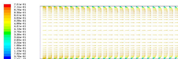
Fig. 3 distribution of velocity vectors at the entrance
