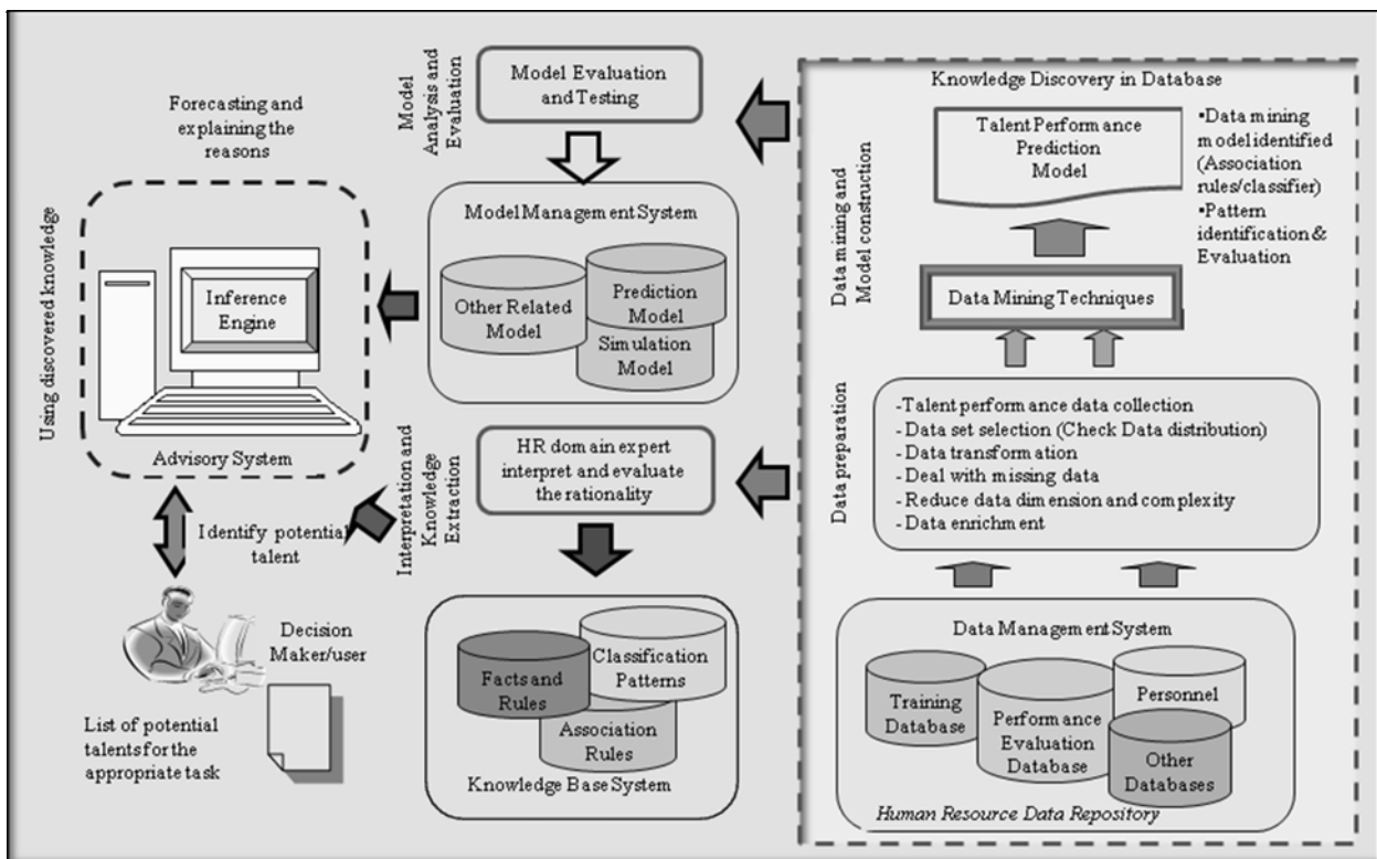
Fig. 5 Suggested HR System Architecture for Talent Forecasting
