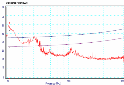
Fig.8 Disturbance Power (System without Filter)
