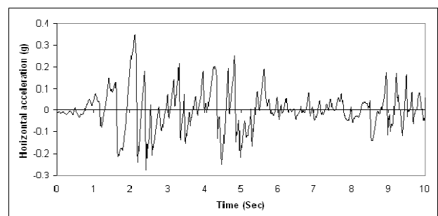
Fig. 3 Horizontal component of the El Centro earthquake
