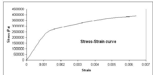
Fig. 2 Multilinear isotropic hardening for material model
