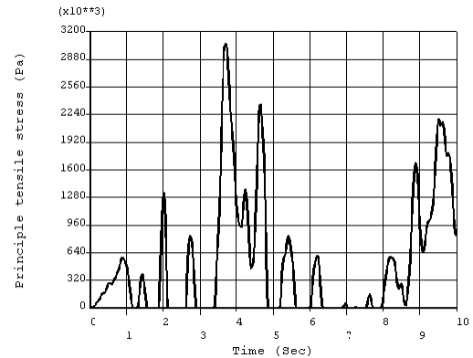
Fig. 7 Time history of principle tensile stress on the bottom of shear wall
