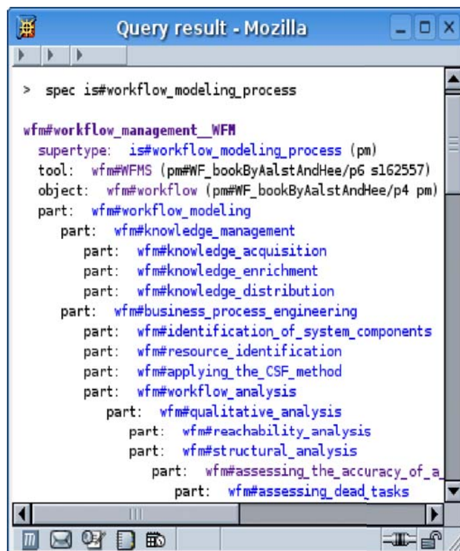
Fig. 2 Command to display the specializations of a type, followed by its first result: wfm#workflow_management (here, this type is displayed along with some of its related objects using an informal format looking like FL).
