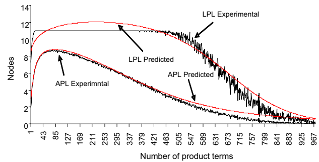
Fig. 1 Comparison of APL and LPL complexity for 10 variables from simulations and NNM predictions
