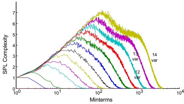
Fig. 3 SPL complexity curves for 2-14 variables after logarithmic transformation is applied to minterms
