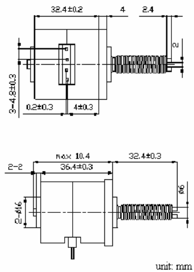
Fig. 4 Geometry of a micro motor
