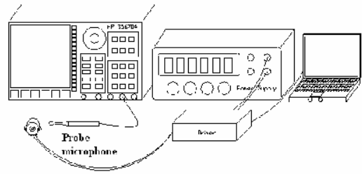
(b) Noise measurement using probe microphone
