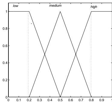
Fig. 2. Membership function.
