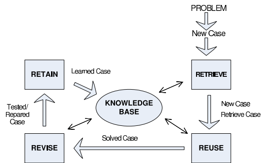
Fig. 1. CBR-Cycle.
