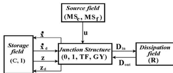
Fig. 1. Key vectors of a bond graph.
