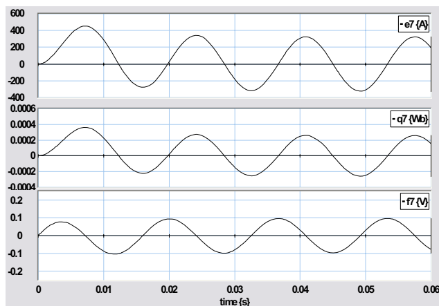
Fig. 8. Magnetic information of the mutual permeance.
