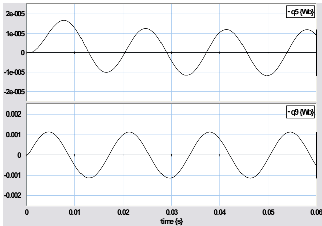
Fig. 9. Leakage fluxes of the transformer.
