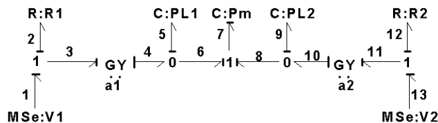
Fig. 7. Magnetic bond graph of the transformer.
