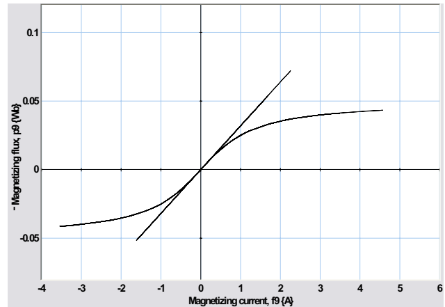
Fig. 9. Nonlinear performance of the transformer of Fig. 4.
