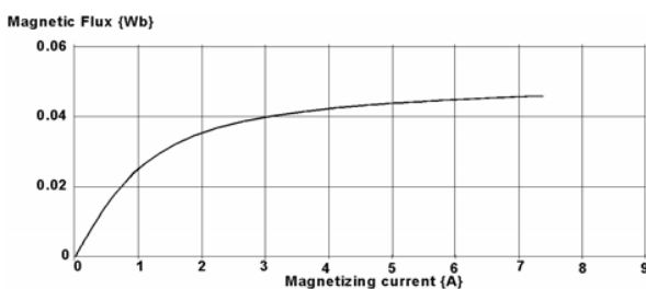
Fig. 8. Saturation curve of equation (48).
