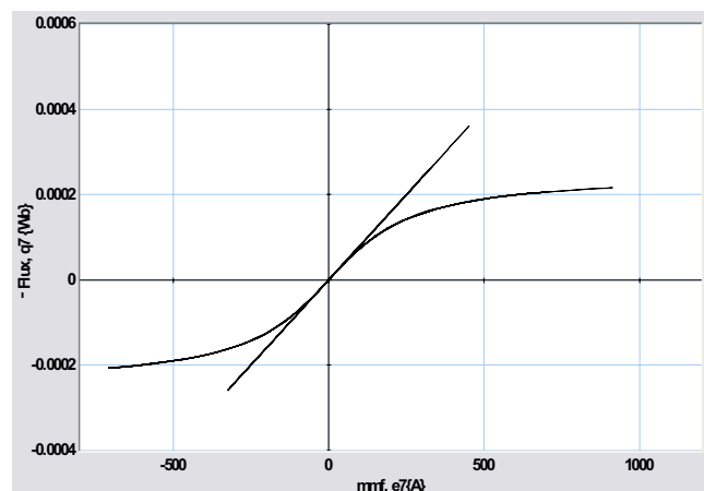
Fig. 10. Nonlinear performance of the transformer of Fig. 7.
