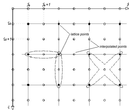
Fig. 1 Lattice scheme
