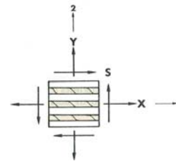
Fig. 3 Definition of fundamental strengths for unidirectional lamina.
