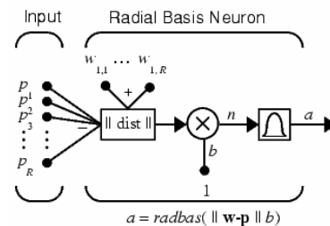
Fig. 9 RBF networks architecture and a simple neuron [9].
