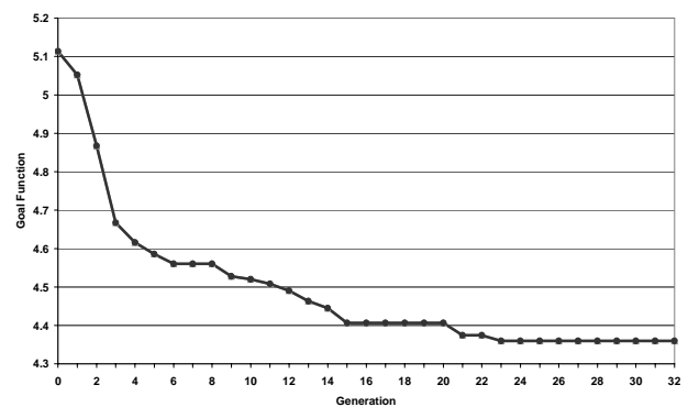
Fig. 12 A convergence history of the multi-objective variations with generations for Example (3).
