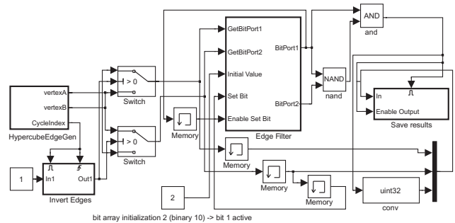
Fig. 4. Block to calculate first tree on Q_4
