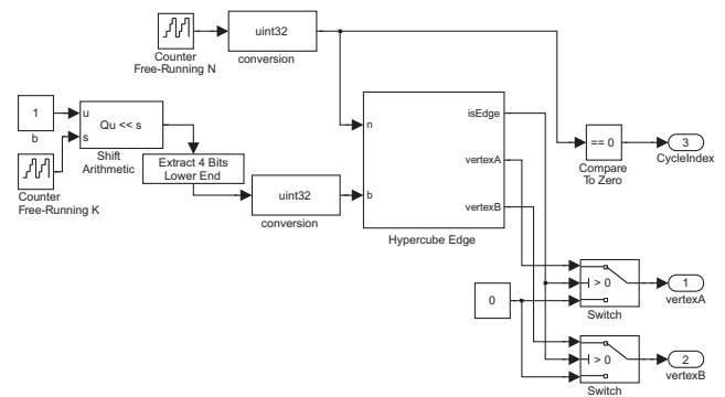
Fig. 5. Hypercube edges build block
