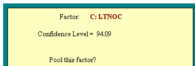
Fig. 13 (a) Pooling of factor C
