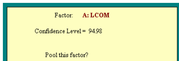
Fig. 13 (b) Pooling of factor A
