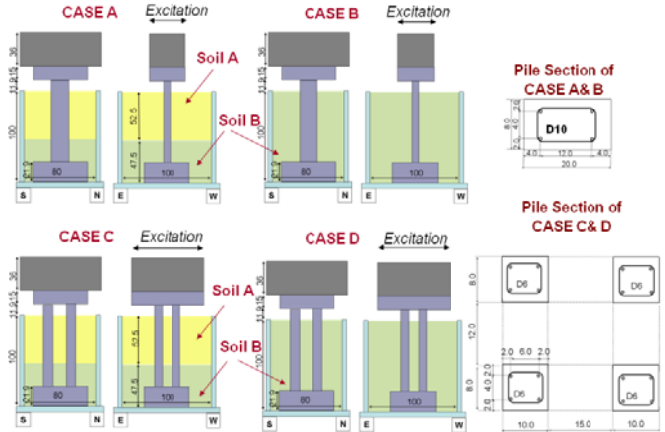
(b) Experimental studied cases and the pile section Fig. 12 Small scale shaking table test properties [6]
