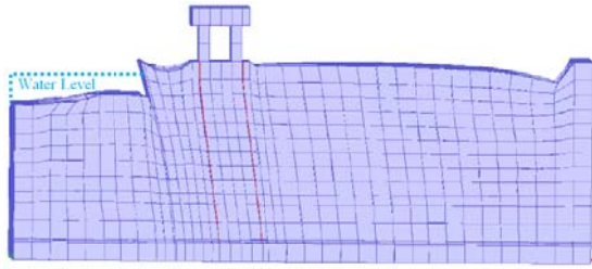
Fig. 9 The lateral deformation of the analytical model
