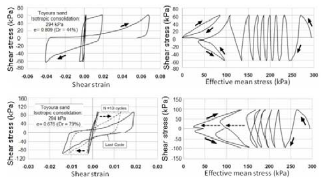
(a) Shear stress strain relation of Toyoura sand under undrained condition (after Towhata 2008[3]) Upper: loose sand, Lower: densely compacted sand
