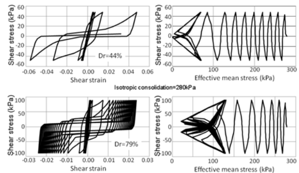
(b) Computed shear stress strain relation under undrained condition Upper: loose sand, Lower: densely compacted sand
