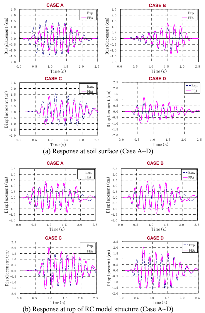
Fig. 17 Comparison of calculated displacement response with experimental data
