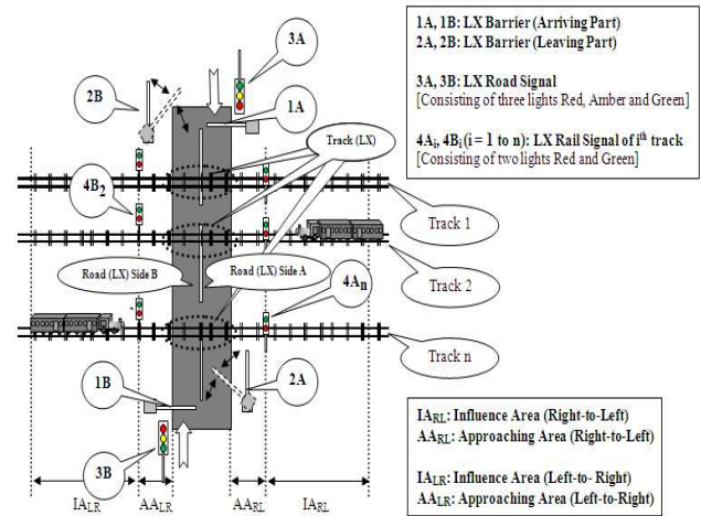
Fig. 1 Description of Multi-Track Railway Level Crossing
