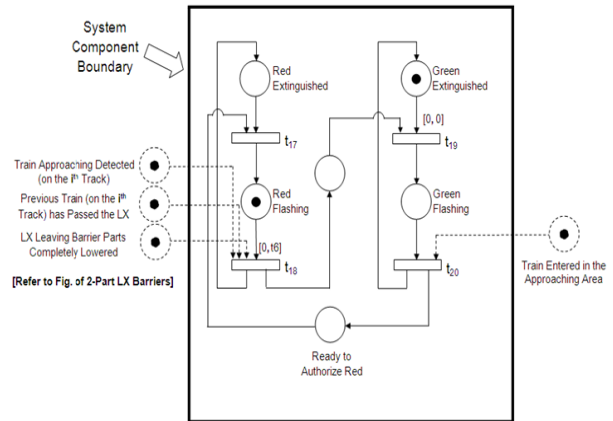
Fig. 4 Timed Petri Net Model of LX Rail Signal of the i^{\text{th}} Track ( i runs from 1 to n )
