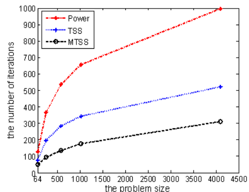
Fig. 3. Comparisons of the iteration counts for the Power, TSS and MTSS iteration methods with the different sized tandem queuing networks.
