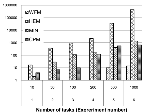
Fig. 7 Logarithmic Runtime for nprocs=8
