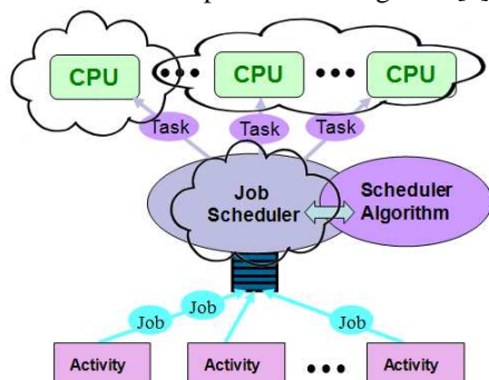
Fig. 1 Simulation Model for meta-scheduling in Clouds
