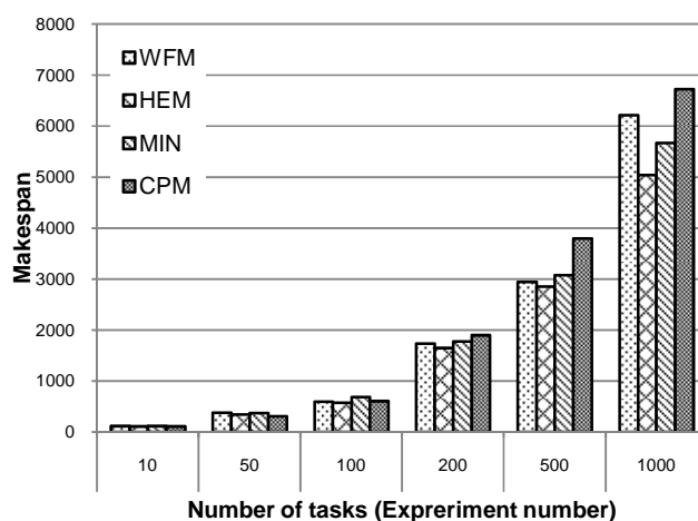
Fig. 6 Makespan Comparison for nprocs = 8
