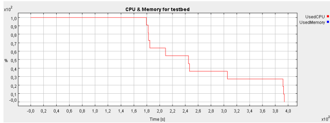
Fig. 9 Simple FCFS Scheduler (100 jobs)
