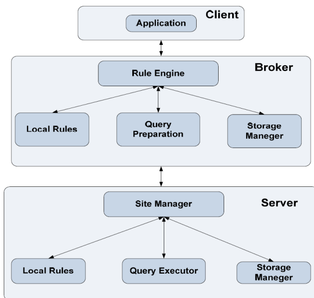
Fig. 3 Distributed approach of simulation model
