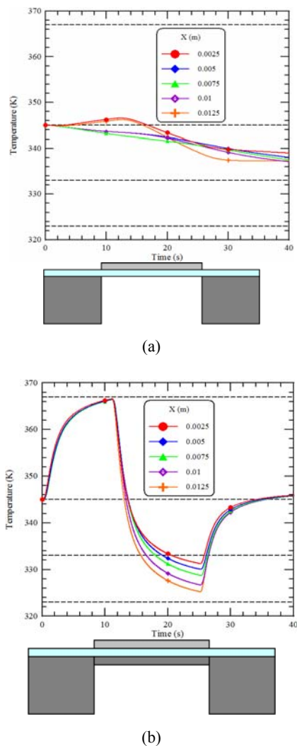
Fig. 9 The temperature distributions at the X-cut cross section at half the chip's length
