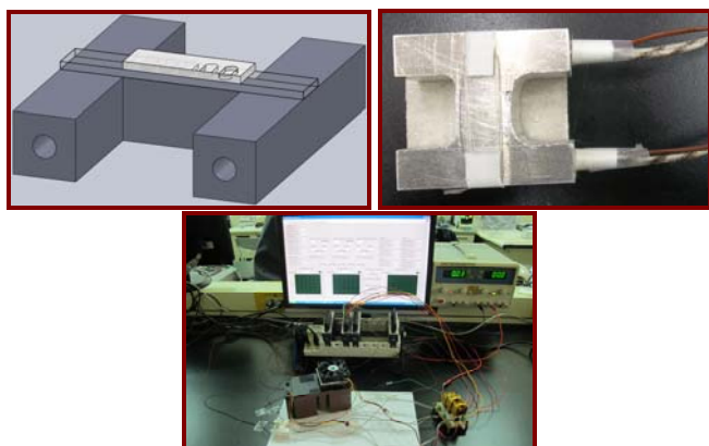
Fig. 2 The experimental setup of the designed system
