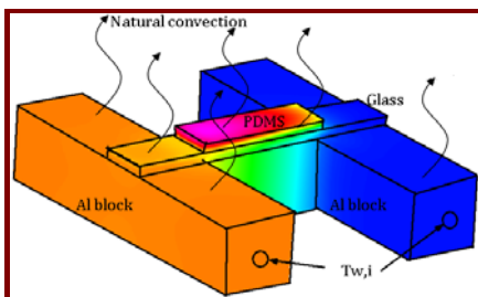
Fig. 1 The physical configuration of the chip
