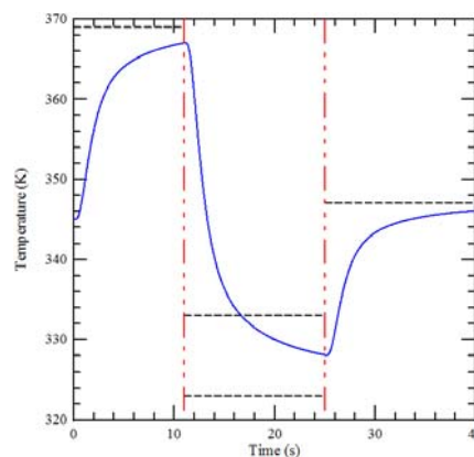
Fig. 4 The center temperature profile of the chamber
