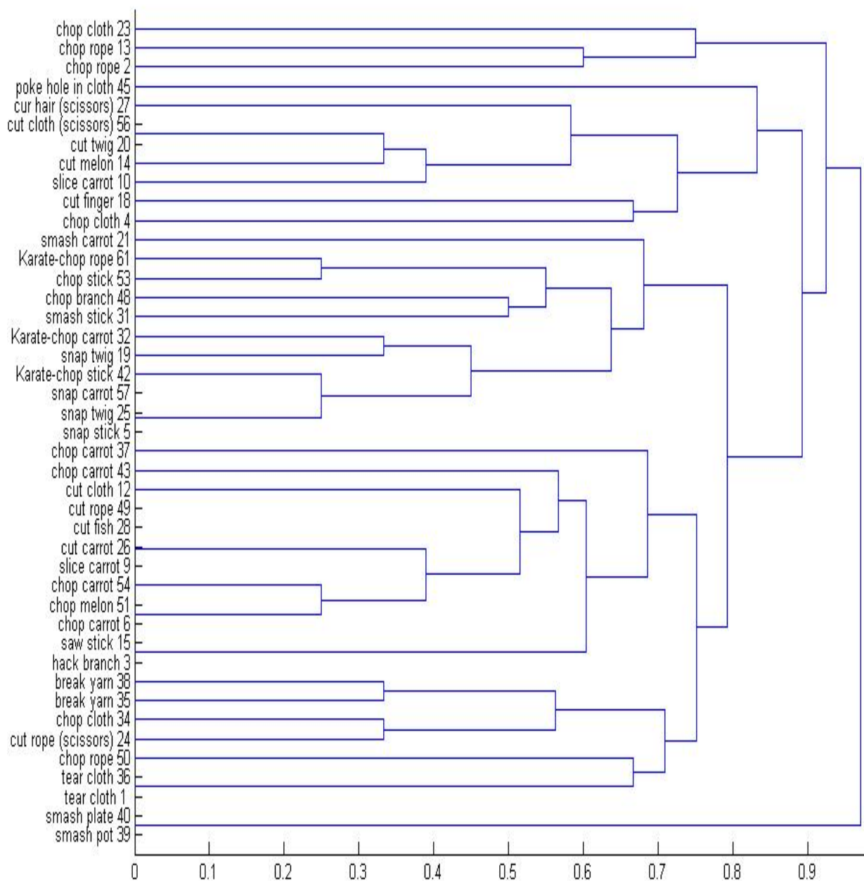
Fig. 2 Telugu Dendrogram
