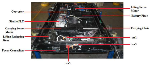
Fig. 6 Top view of the shuttle robot
