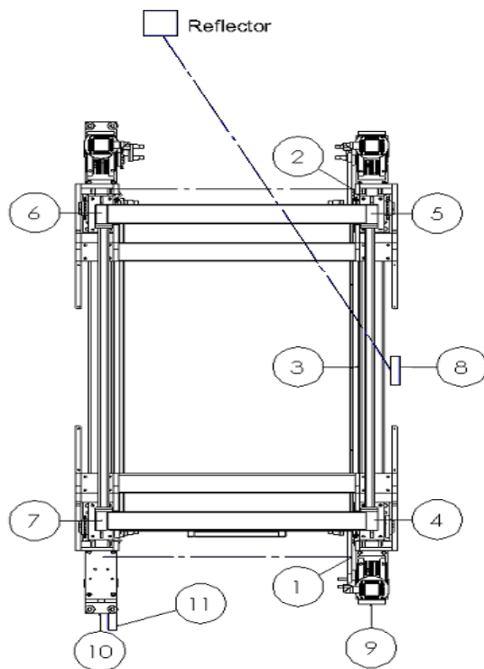
Fig. 4 Aisle robot and sensor positions (top view)
