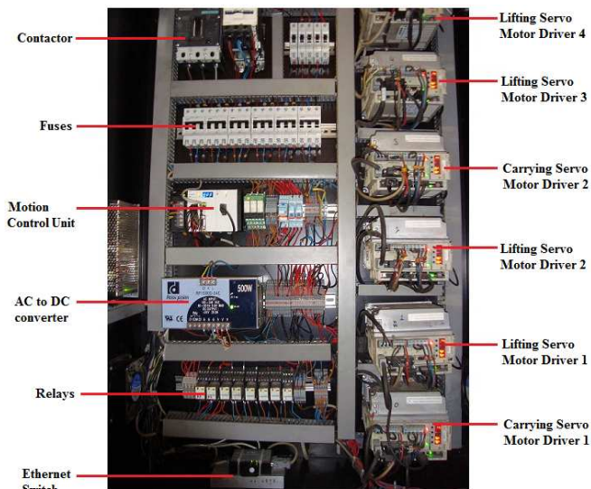
Fig. 10 Aisle Robot Control Panel
