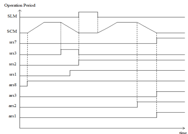
Fig. 5 Shuttle robot operation period graph
