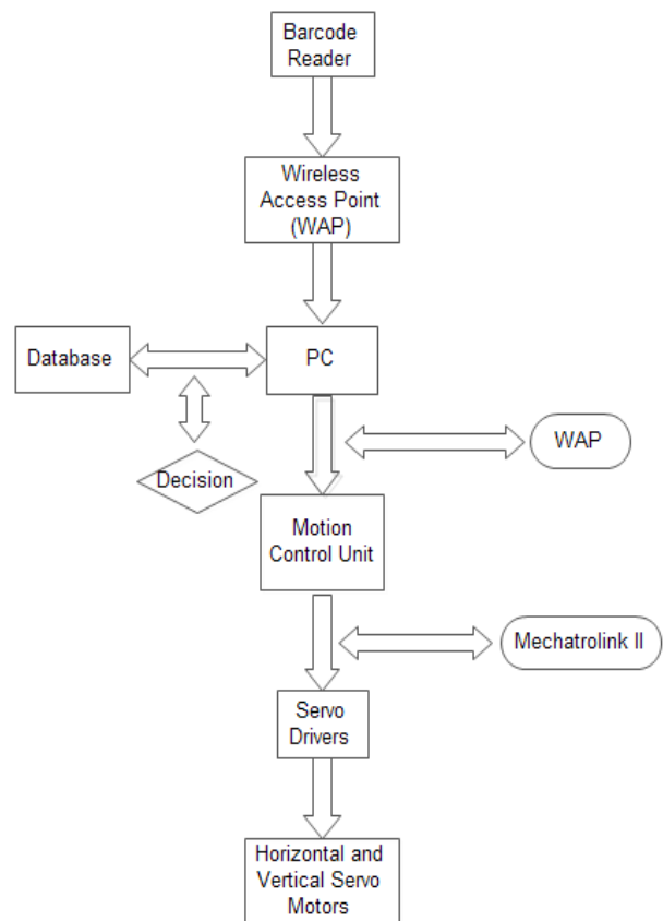
Fig. 9 Aisle robot schematic diagram
