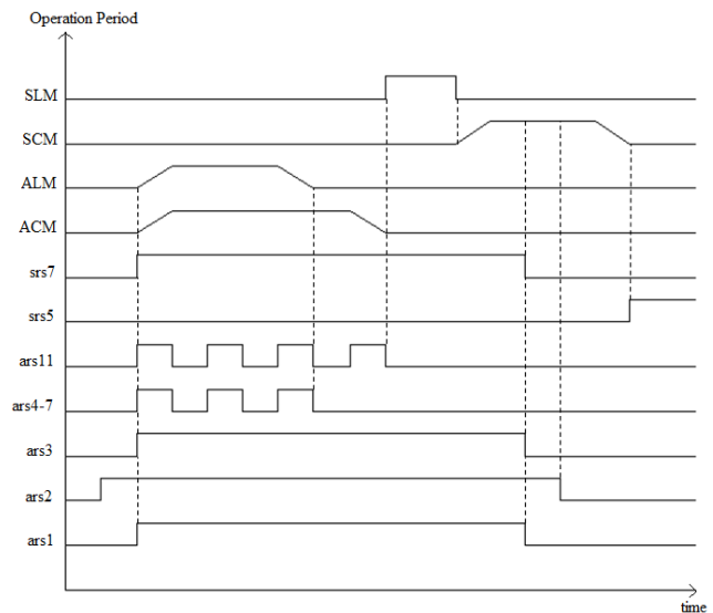
Fig. 8 Aisle robot operation period graph
