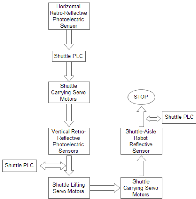
Fig. 7 Shuttle robot schematic diagram
