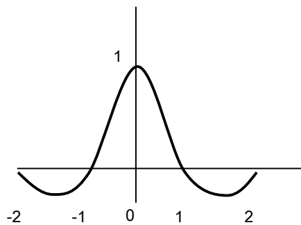
Fig. 1 Catmull-rom spline interpolation kernel
