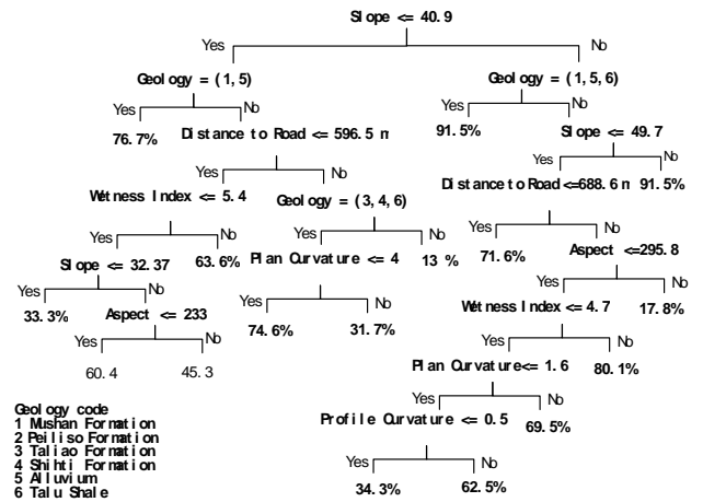
Fig. 2. Graphical representation of the landslide tree model.
